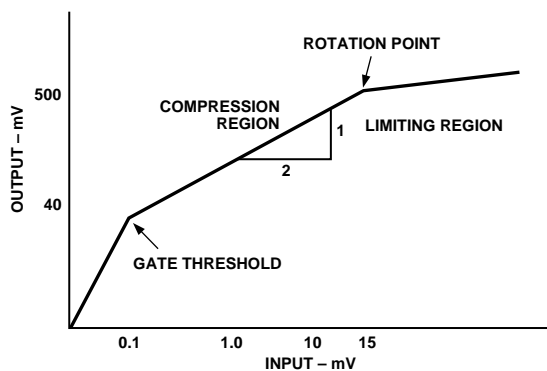
Figure 25. Transfer Characteristic
