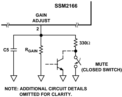
Figure 19. Details of SSM2166 Mute Option
