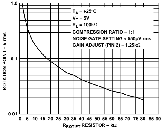
Figure 9. Rotation Point vs. R ROT PT (Pin 11 to V + )
