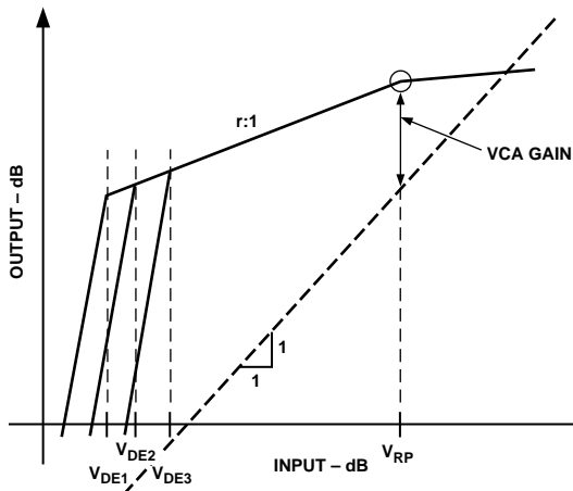
Figure 20. Effect of Varying the Downward Expansion (Noise Gate) Threshold
