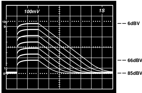
Figure 15b. RMS Level Detector Performance with C_{AVG} = 22 \mu F
